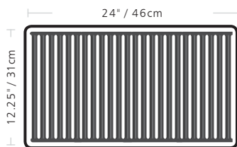
Cast Iron Grid PORTA-CHEF™ 320
