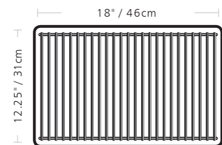
Porcelain Coated Steel Grid PORTA-CHEF™ 100
