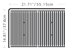
Cast Iron Grids
