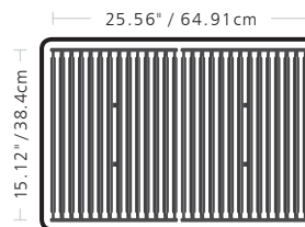
Cast Iron Grids SIGNET™ SERIES
