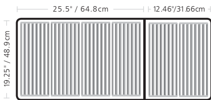
Cast Stainless Steel Grids IMPERIAL™ XL
