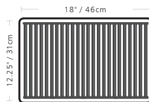
Cast Iron Grid PORTA-CHEF™ 120
