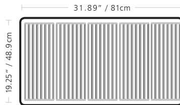
Cast Stainless Steel Grids IMPERIAL™ 590
