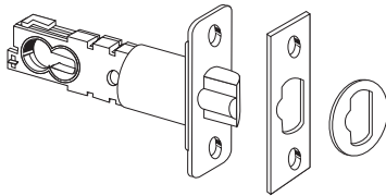
TRIPLE OPTION DEADLATCH
